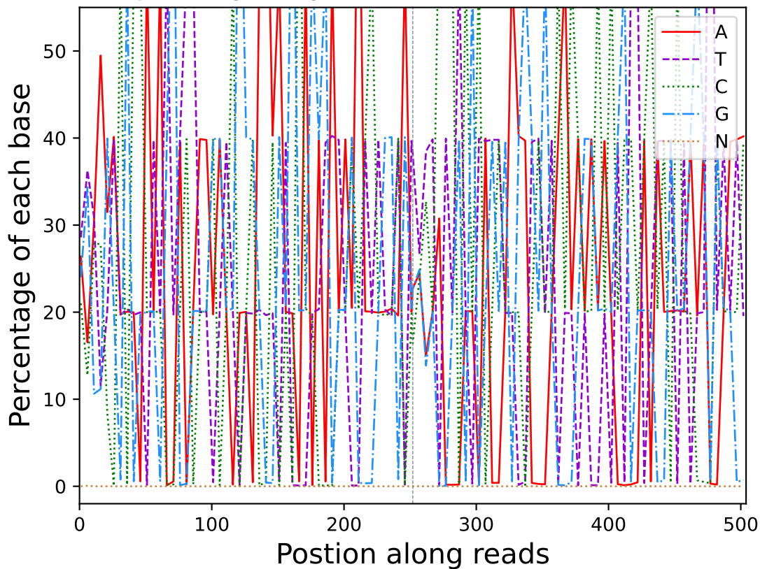
Base percentage along reads (R10212)
